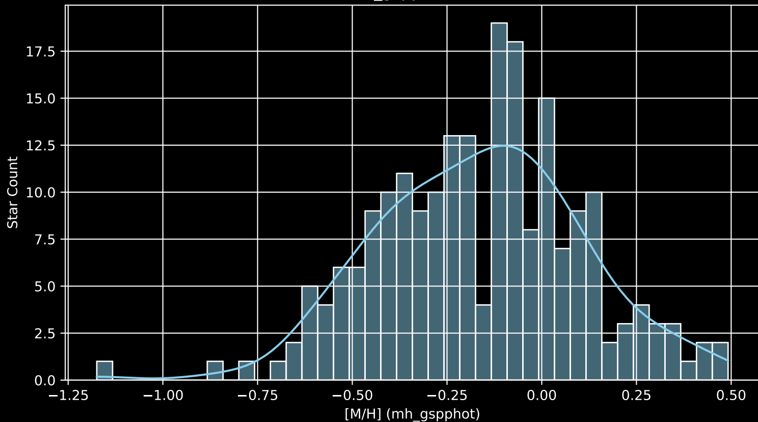
APOGEE DR17 Field: [269-37-O_TESS [M/H] (mh_gspphot) (n= 212)
