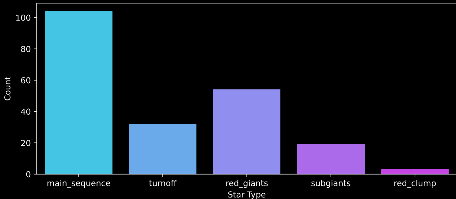
APOGEE DR17 Field: [269-37-O_TESS] Count plot of Star Type
