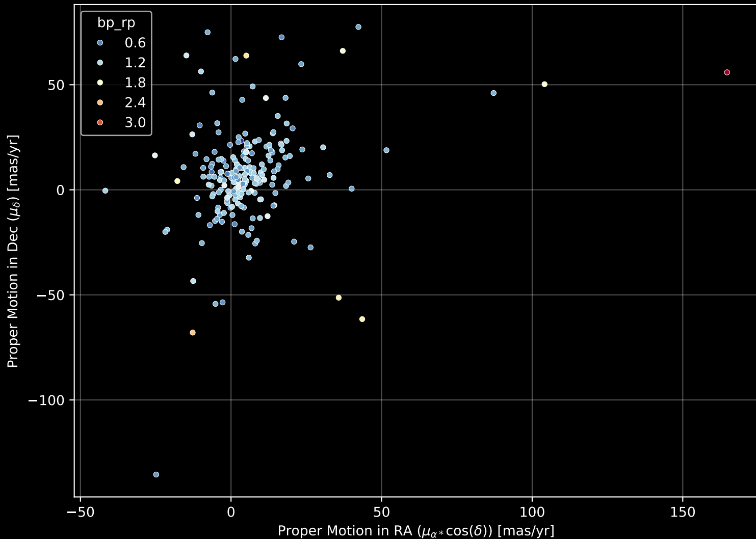
APOGEE DR17 Field: [269-37-O_TESS] Proper Motion Diagram (n= 212)
