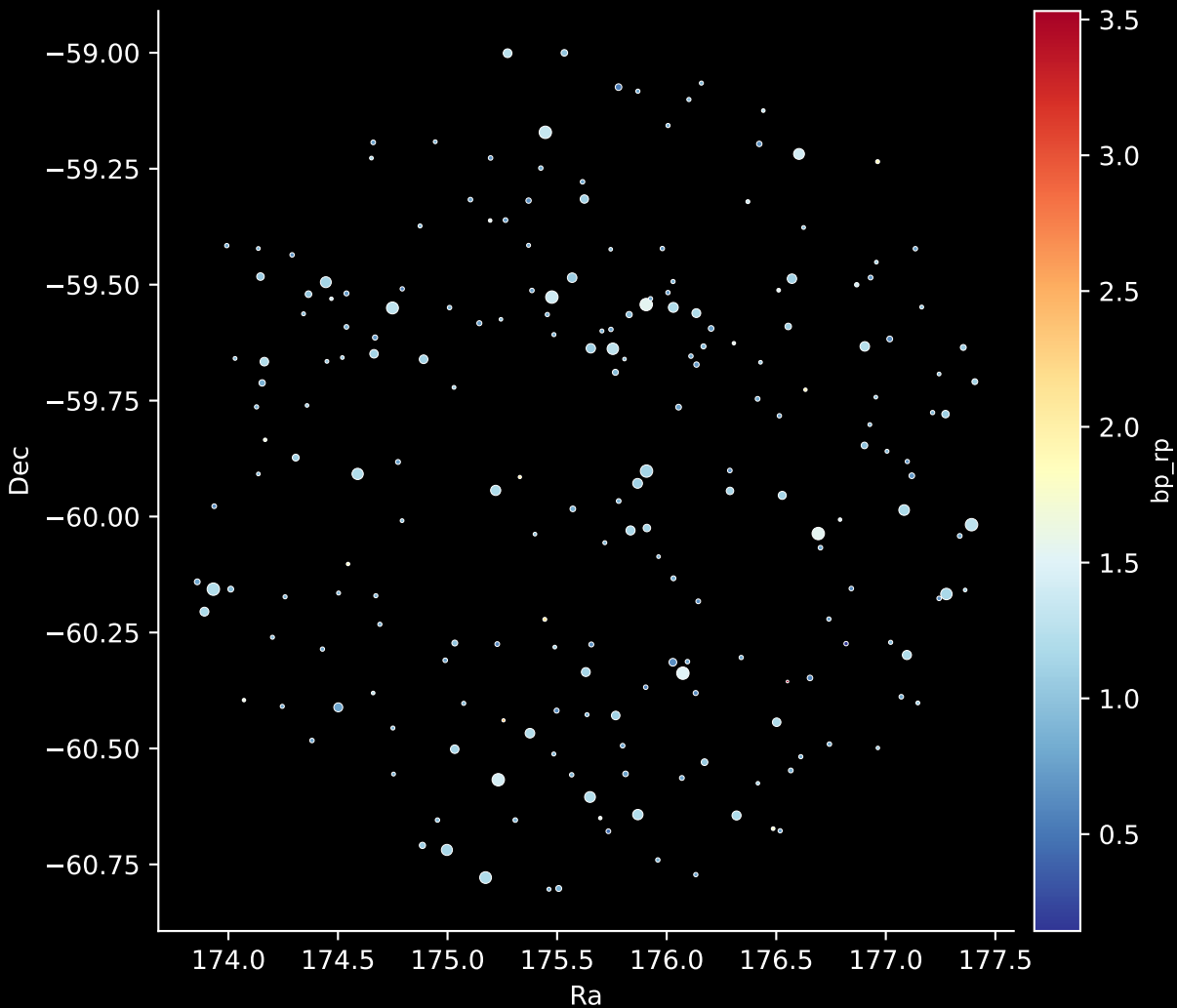
APOGEE DR17 Field: [269-37-O_TESS] Stars: 212
