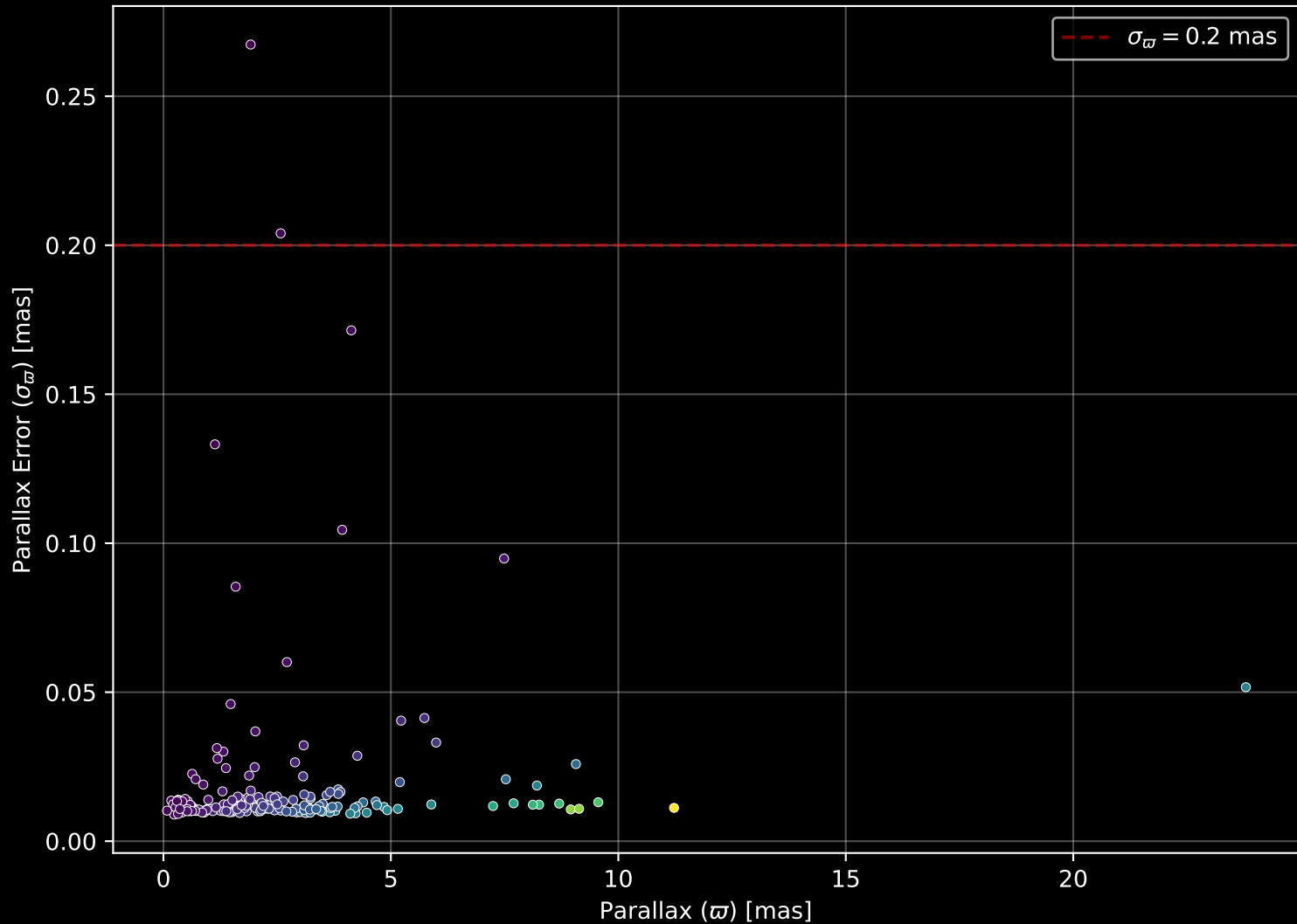
APOGEE DR17 Field: [269-37-O_TESS] Parallax Quality (n= 212)
