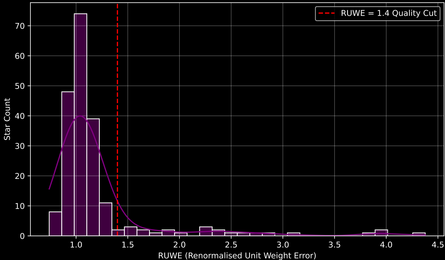
GAPOGEE DR17 Field [269-37-O_TESS] RUWE Distribution (n= 205)
